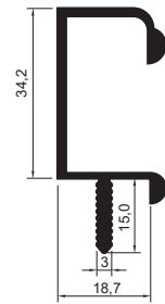
18 mm Suntalam / chipboard
