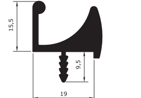
18 - 19 mm Suntalam / chipboard
