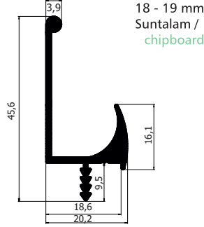
18 - 19 mm Suntalam / chipboard
