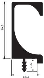
18 mm Suntalam / chipboard
