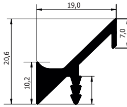
18 - 19 mm Suntalam / chipboard
